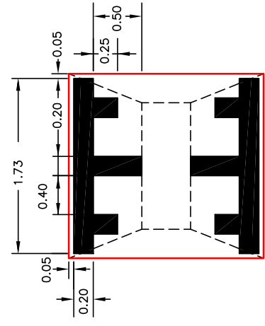
LINEMARKING DETAIL
