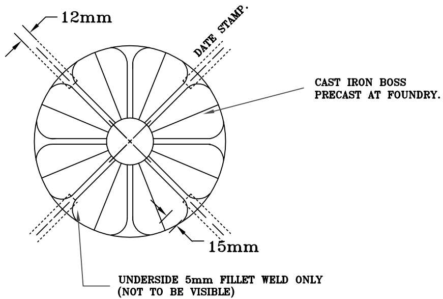
FRONT ELEVATION DETAIL C
